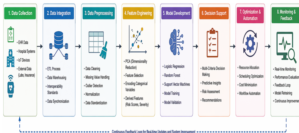
Figure 2: Multistage Workflow of Automated Healthcare Decision System
